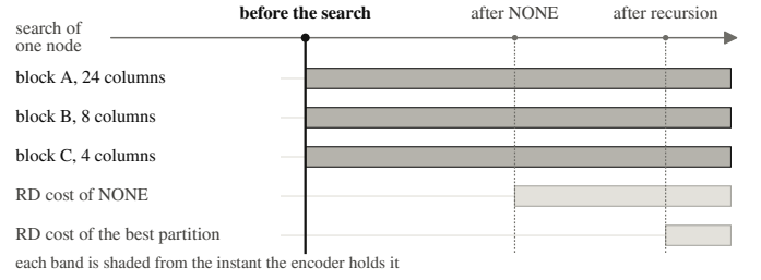
Fig. 1. Information available to a pruner at each instant of the search of a partition node. Each band is shaded from the instant the encoder holds it, so the three column blocks are free at the pre-search instant addressed in this work, while the rate-distortion costs are not yet defined there.
