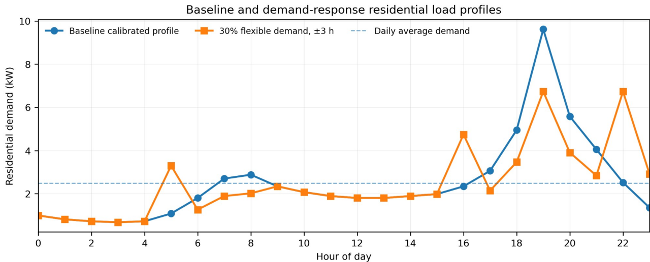
Figure 2. Baseline calibrated residential profile and optimized profile for the 30% flexibility, \pm 3 -hour scenario. Daily energy is conserved.
