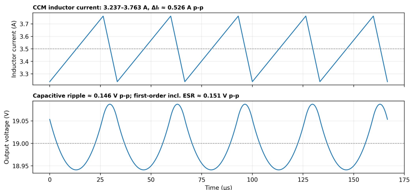
Figure 7. Analytical rated-point ripple. These are reconstructed theoretical waveforms from the documented L , C , \text{ESR} , f_s , V_{in} and V_o ; they are not digitized measurements from the archived MATLAB figure.
