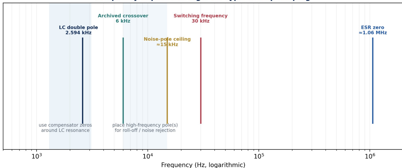
Figure 7. Frequency-separation map. The 2.594 kHz LC resonance and 6 kHz crossover dominate the useful loop-shaping range; the 1.06 MHz ESR zero lies far beyond switching frequency.
