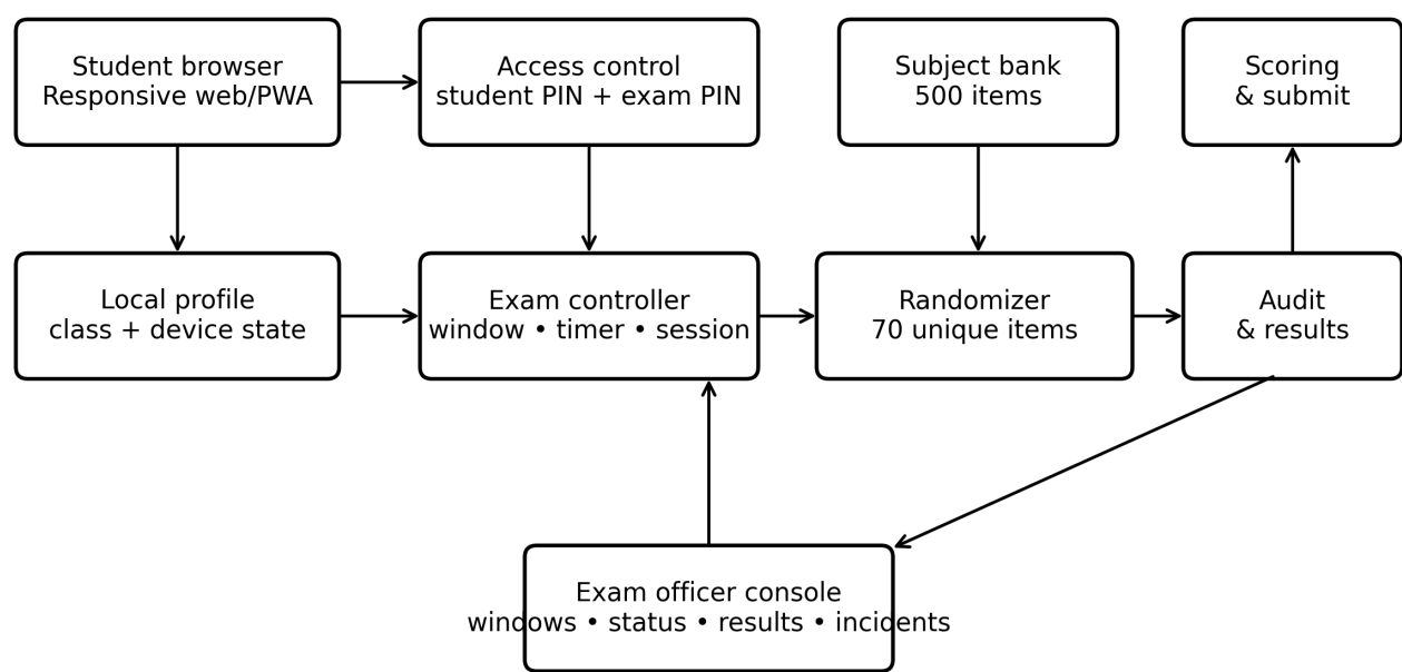
CACGWA Student Revision and CBT Portal — logical architecture
