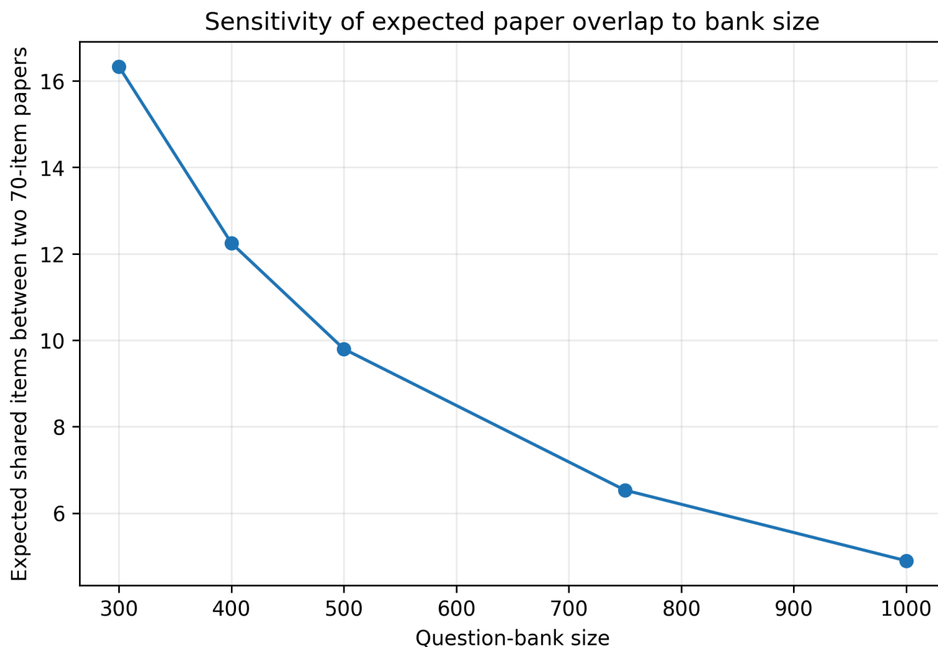
Figure 5. Expected pairwise overlap falls rapidly as the item bank becomes larger.
