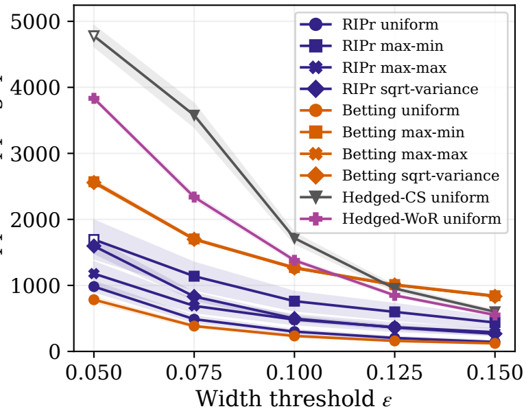
Mean capped stopping queries
