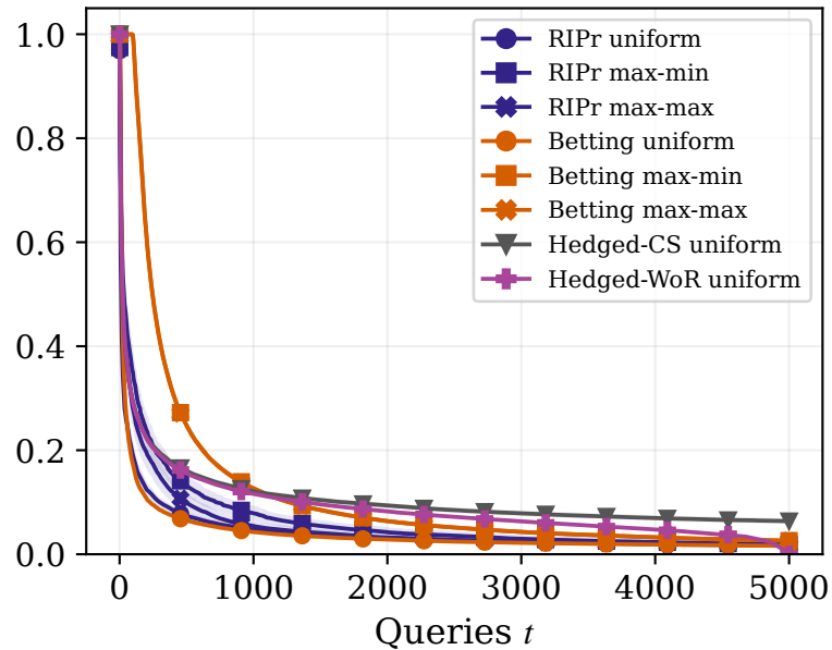
Mean CS width
