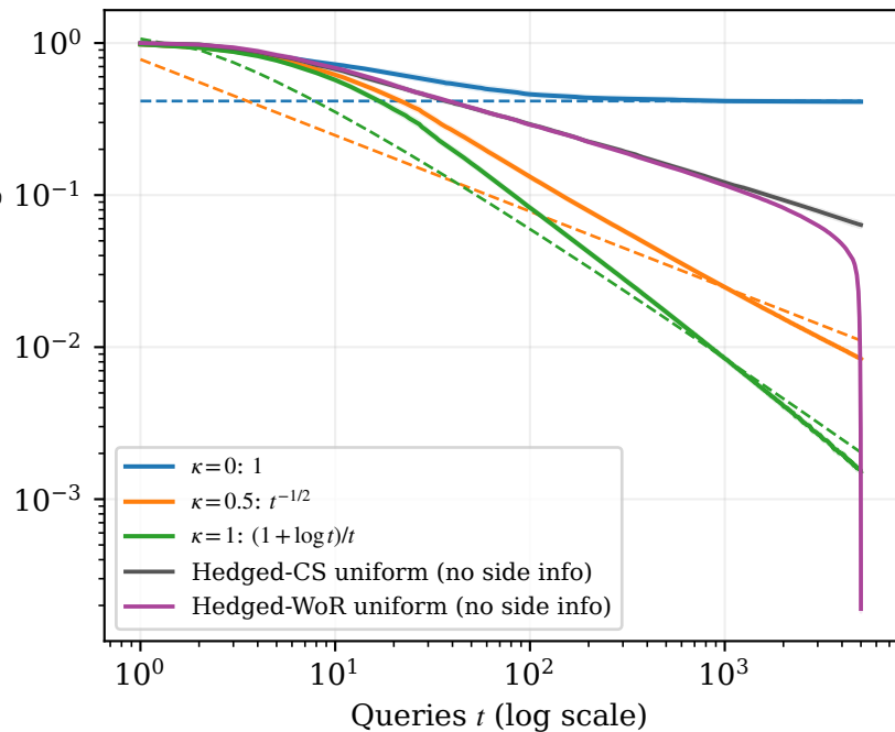
Mean RPr-CS width (log scale)
