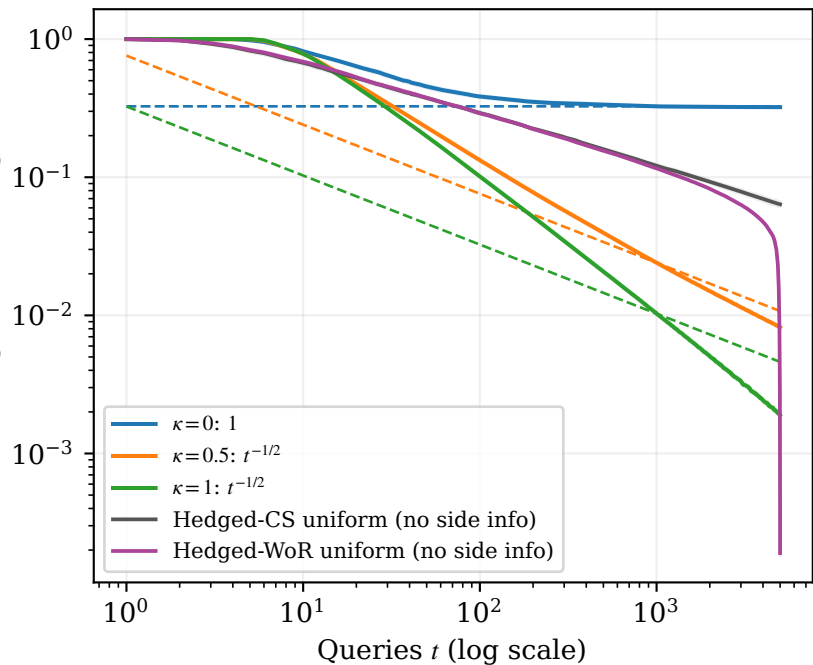
Mean Betting-CS width (log scale)
