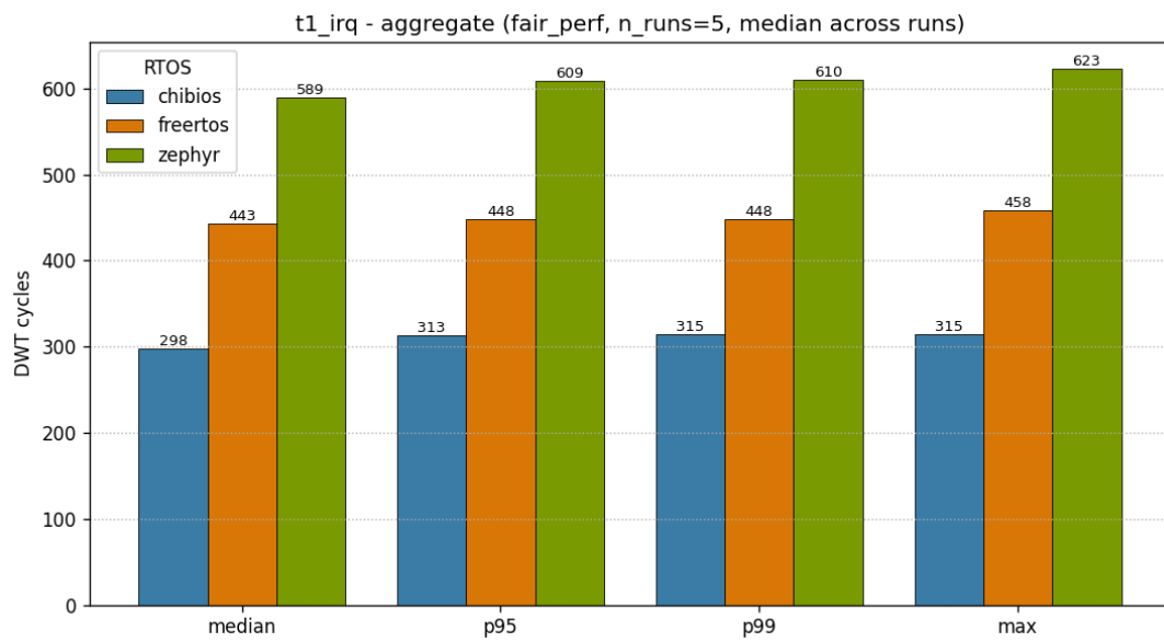
Aggregate distribution - fair_perf / t1_irq
