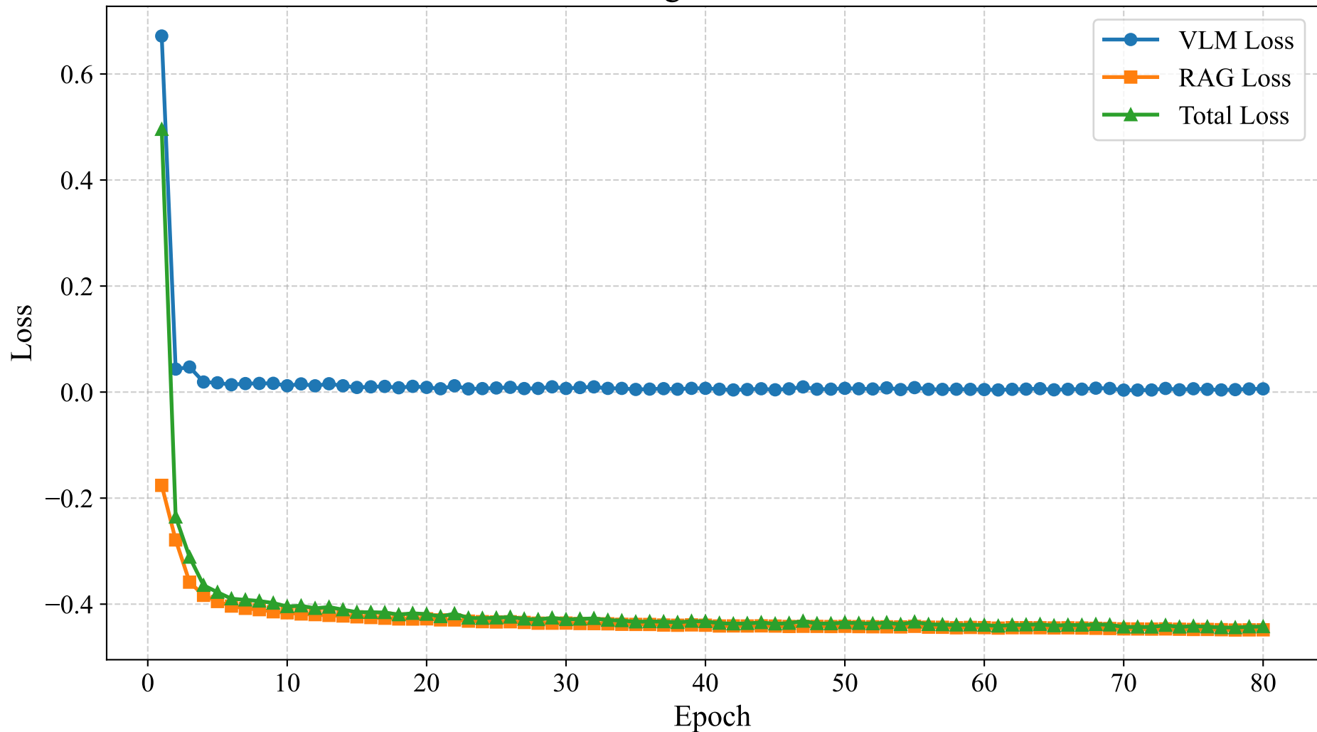
Training Loss Curves
