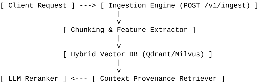
Figure 1: High-Level Vector Ingestion and RAG Query Pipeline
