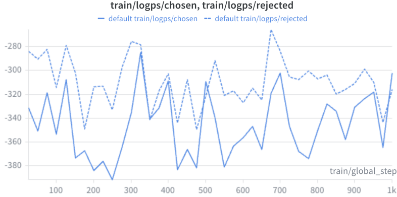
Figure 7: logps/chosen (solid) and logps/rejected (dashed), train — raw policy log-probs \log \pi_\theta(y \mid x) (not log-ratios). Chosen sits below rejected mainly because chosen responses are longer (271.9 vs 245.4 tokens), so their summed log-prob is more negative.
