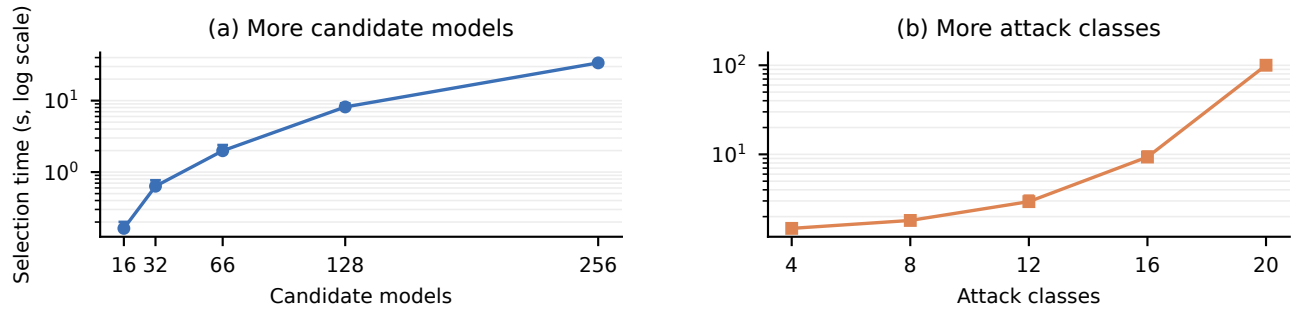
Figure 5. Exact selection time in two independently sampled sweeps. Panel (a) fixes 12 attack classes and varies the candidate pool, while panel (b) fixes 66 candidates and varies the attack class count. The vertical axis is logarithmic, and points are medians and upper bars are 95th percentiles over ten repetitions.
