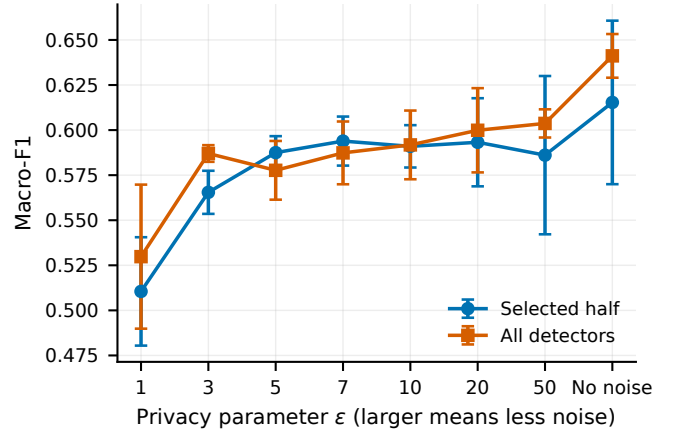
Figure 5. Privacy–utility trade-off under Laplace score randomization. Larger \epsilon means less noise; bars show 95% confidence intervals over the same five DDoS splits.
