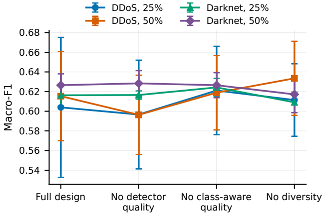
Figure 4. Macro-F1 for the full design and one-at-a-time removals of detector quality, class-aware quality, and prediction diversity. Bars show 95% confidence intervals over five splits.
