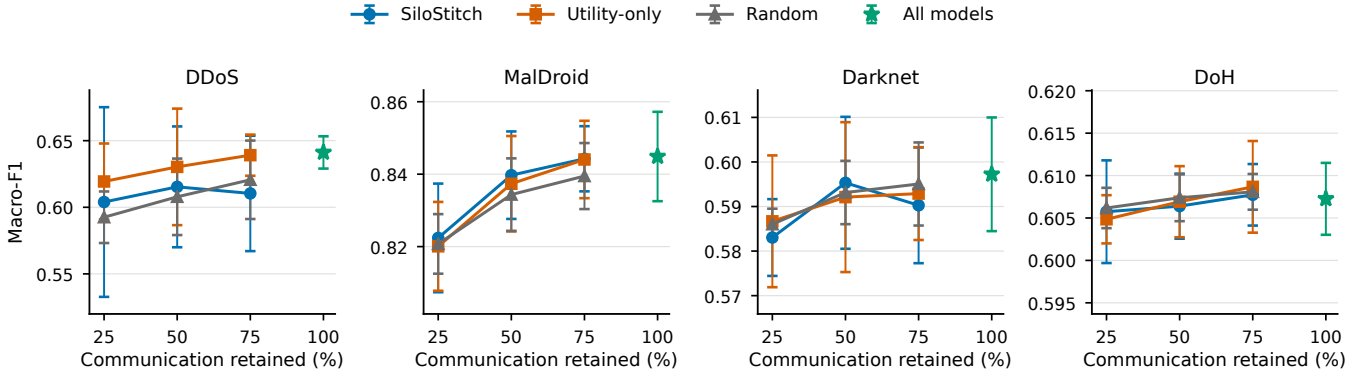
Figure 2. Detection quality as communication changes. Lines follow three selection rules at the 25%, 50%, and 75% budgets; the star denotes all 66 models. Error bars are 95% confidence intervals over five repeated splits. Each dataset uses its own vertical scale.
