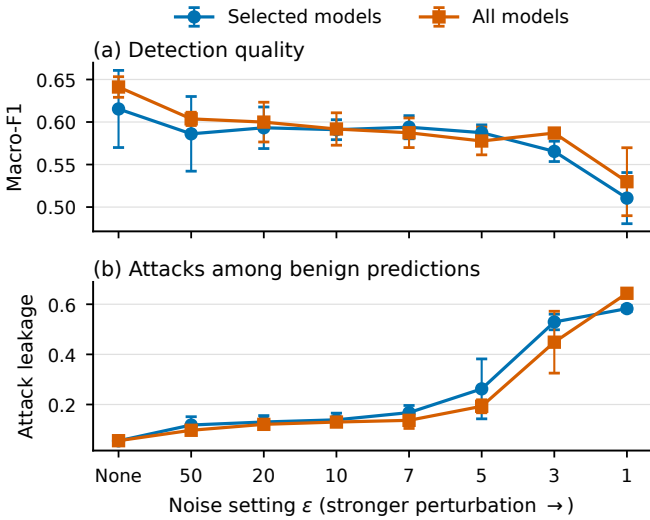
Figure 4. Privacy–utility trade-off under Laplace score randomization. Panel (a) reports aggregate detection quality; panel (b) reports attacks hidden among predictions labeled benign. Larger \epsilon means less noise; error bars show 95% confidence intervals over the same five DDoS splits.
