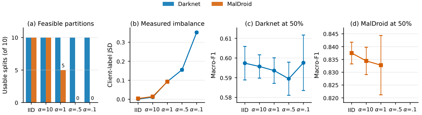
Figure 3. Detection under controlled client-label heterogeneity. (a) counts usable splits among ten attempts at each level; (b) measures the resulting client-label imbalance, where larger JSD means more uneven label mixtures; and (c–d) report Macro-F1 at the 50% communication budget. Confidence intervals use the usable splits ( n = 10 , or n = 5 for MalDroid at \alpha = 1 ).
