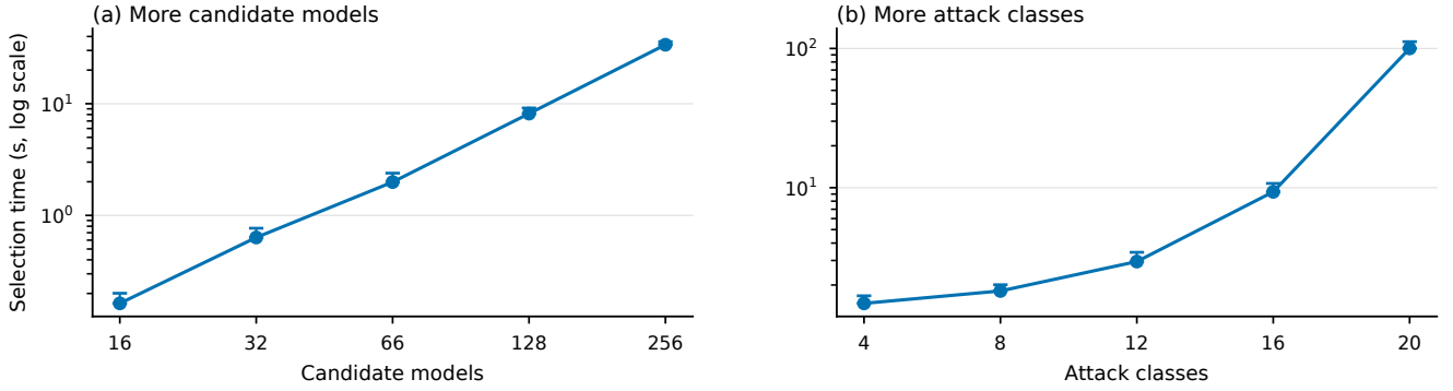
Figure 5. Time required to select models as the deployment grows. The panels independently vary candidate models and attack classes on a logarithmic time scale. Points are medians over ten repeats; upper bars mark the 95th percentile.
