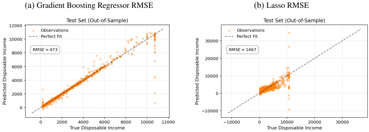
Figure 14: Model Performance
