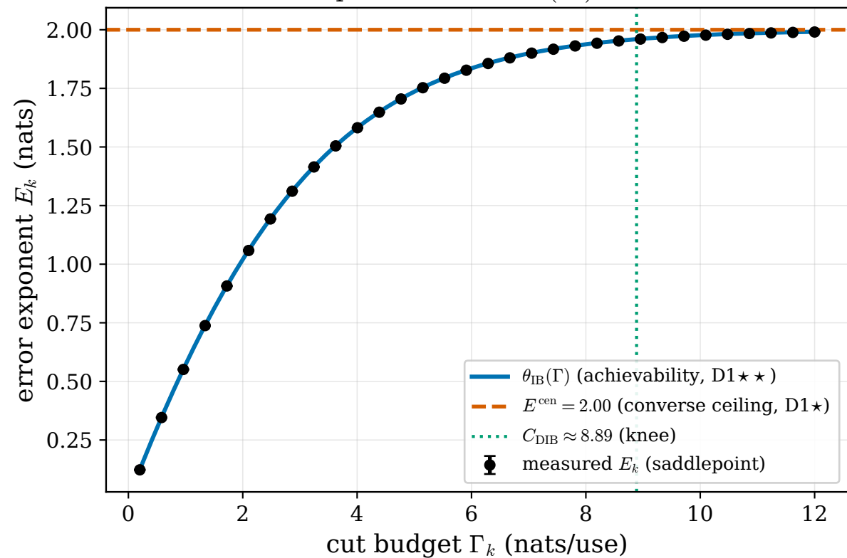
D1-E1: measured exponent tracks \theta_{\text{IB}}(\Gamma_k) under the E^{\text{cen}} ceiling
