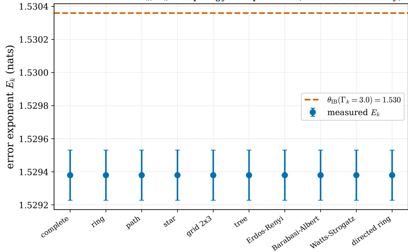
D1-E3: at fixed \Gamma_k , E_k is topology-independent (min-cut sufficiency)
