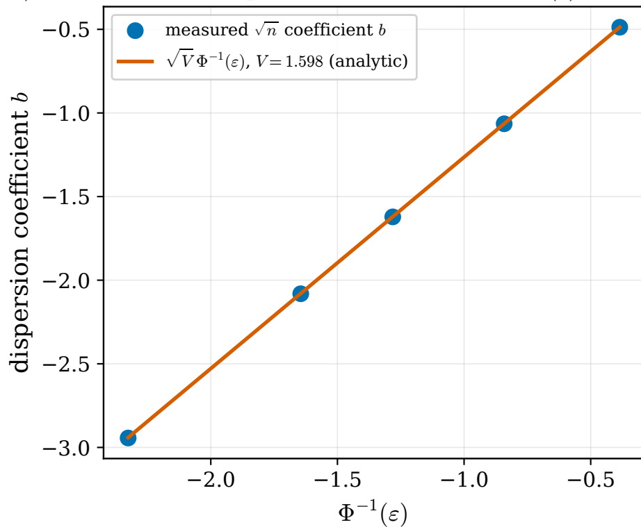
(b) dispersion scales as \sqrt{V}\Phi^{-1}(\varepsilon)
