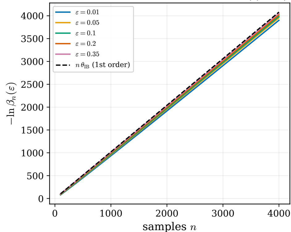
(a) finite- n error: -\ln \beta_n = n\theta_{\text{IB}} - \sqrt{nV}\Phi^{-1}(\varepsilon) + O(\ln n)
