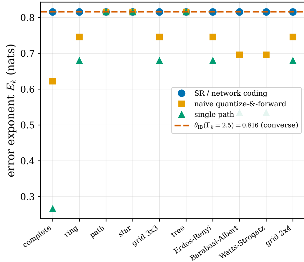
(a) matched min-cut \Gamma_k = 2.5 : SR collapses, naive spreads
