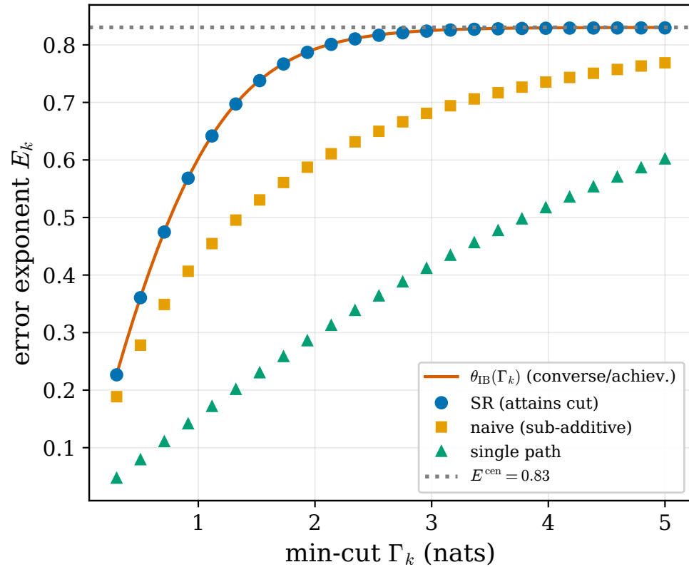
(b) K_6 : only SR attains \theta_{\text{IB}}(\Gamma_k)
