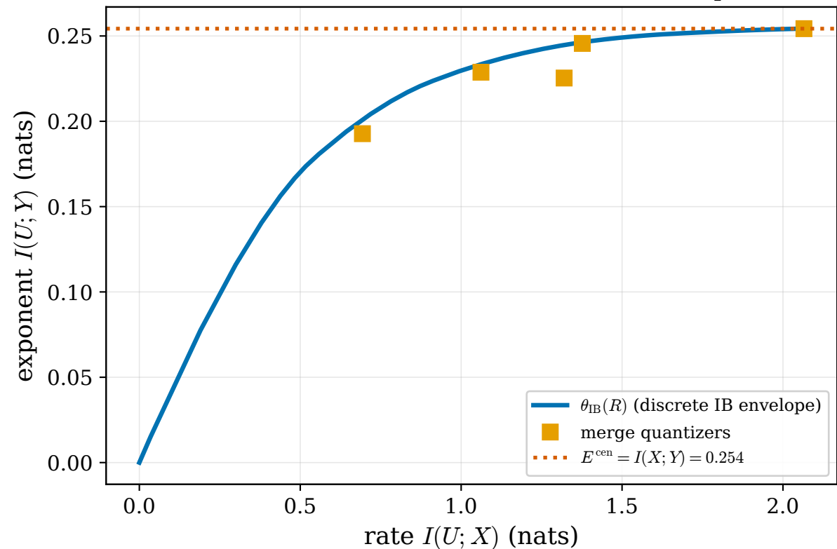
D1-N3: non-Gaussian (discrete) — converse envelope \theta_{\text{IB}} holds
