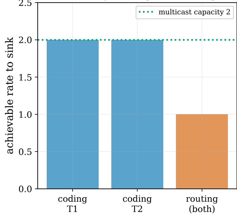
(c) butterfly: coding 2 vs routing 1
