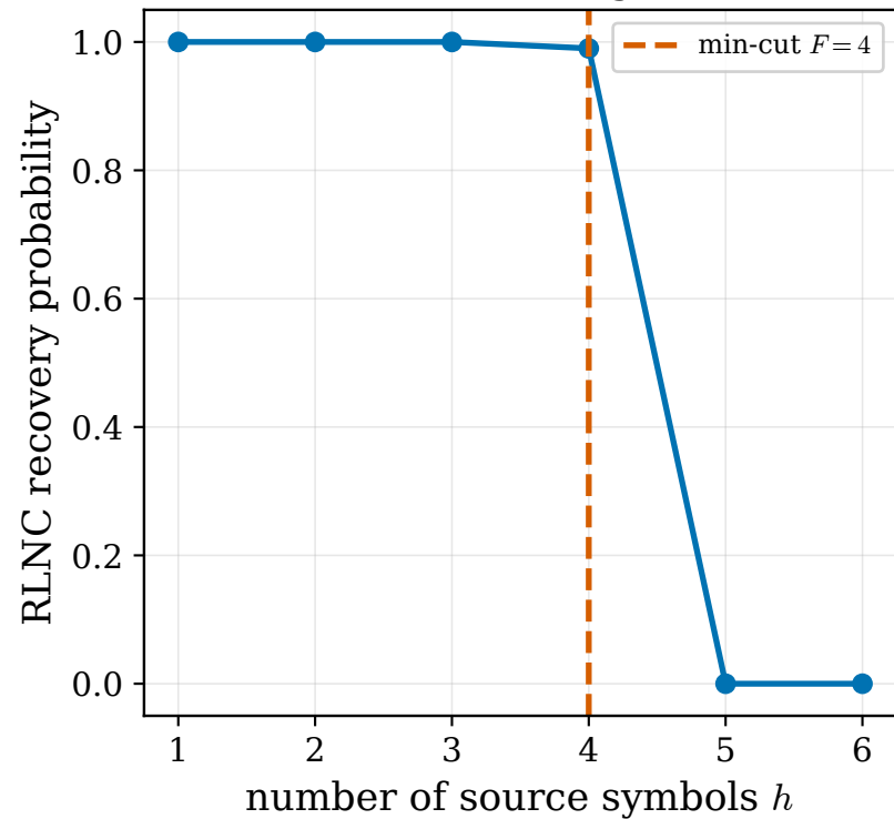
(a) recovers iff h \leq F (grid, q = 257 )
