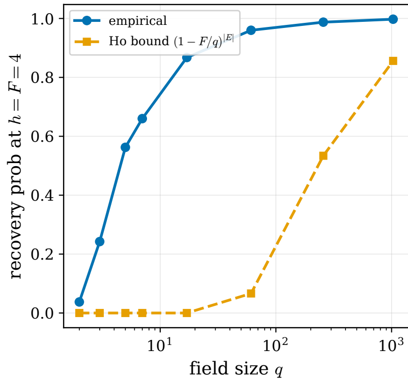
(b) random code \rightarrow 1 as q \rightarrow \infty
