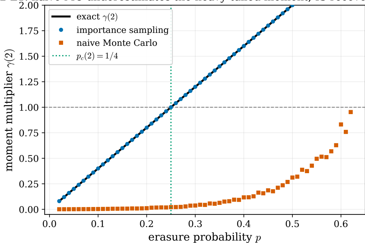
D2-E1: naive MC underestimates the heavy-tailed moment; IS recovers exact \gamma
