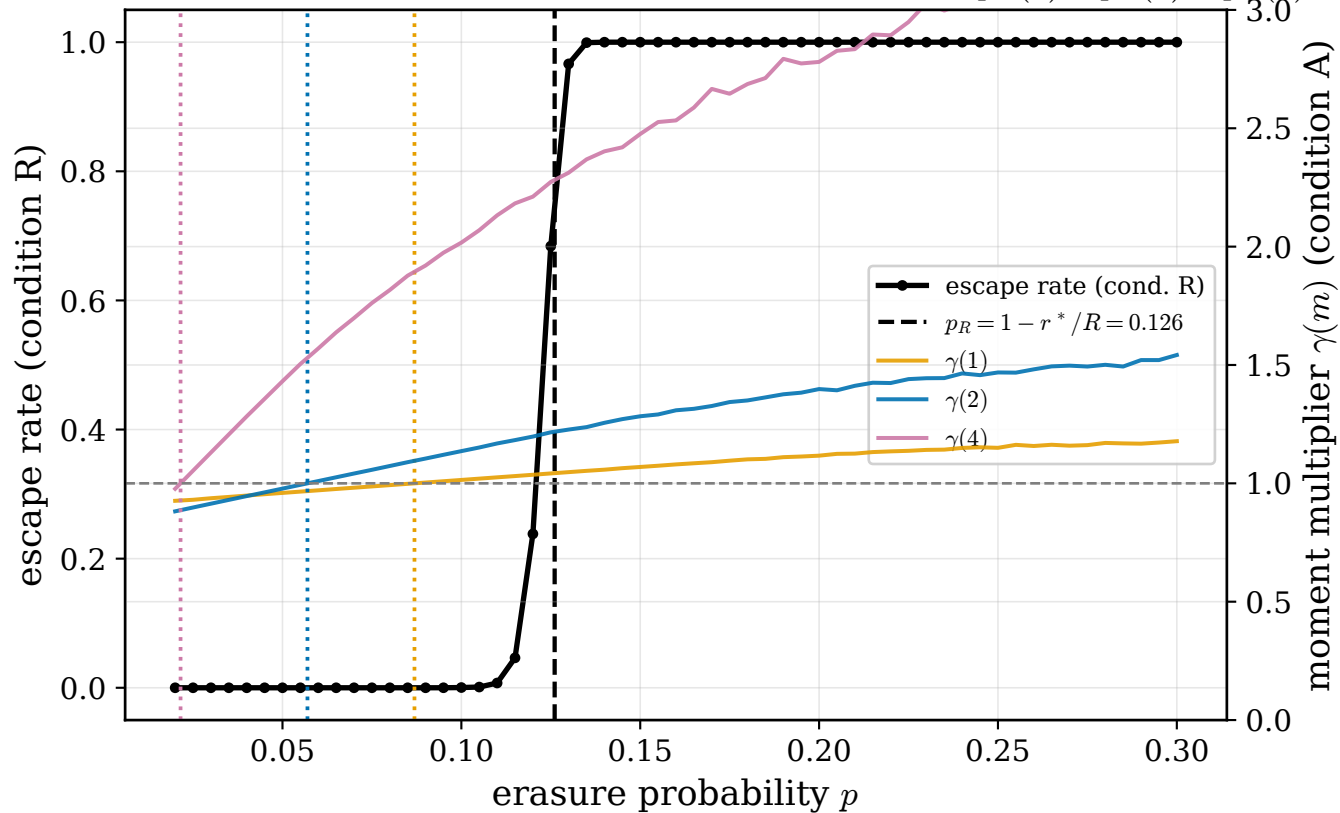
D2-E2: two conditions at R = \ln 2 + 0.1 — moment cascade p_A(4) < p_A(2) < p_A(1) < p_R
