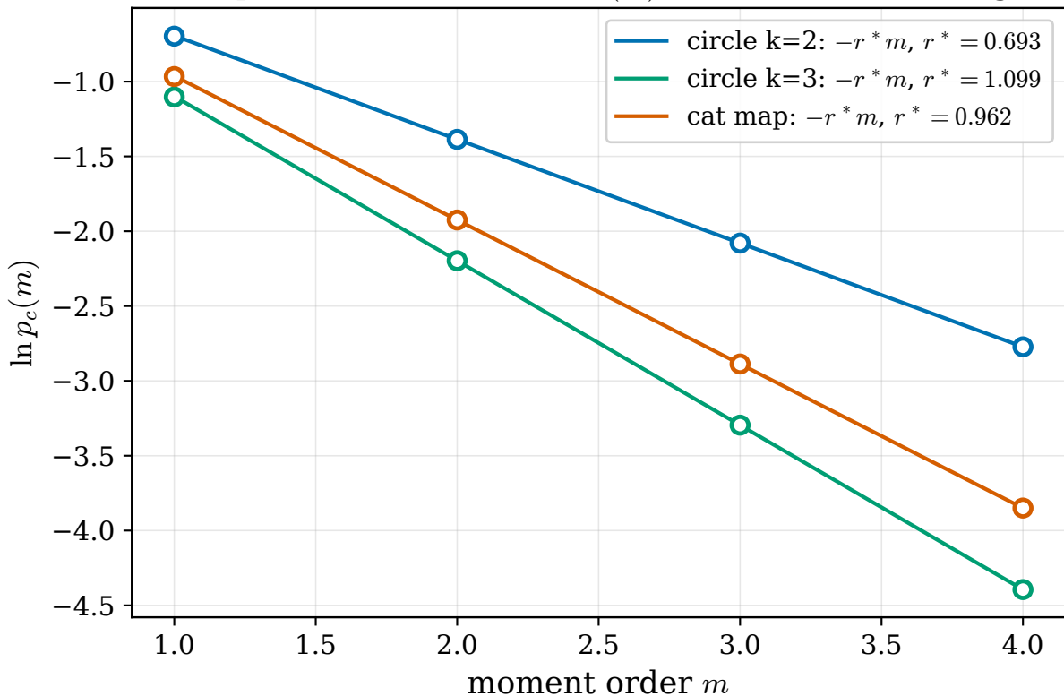
D2-E3: parameter-free law \ln p_c(m) = -r^* m across surrogates
