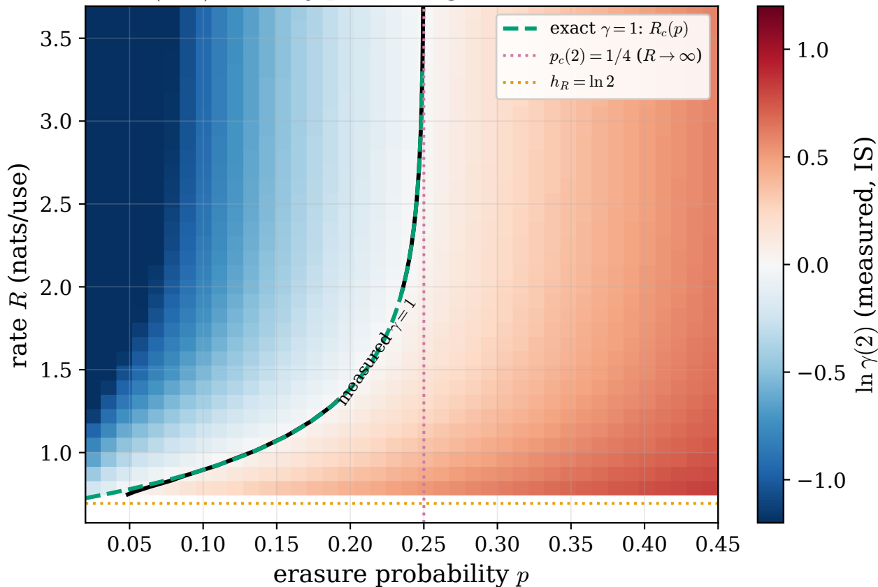
D2-E4: (p, R) stability phase diagram, m = 2 (circle k = 2 )
