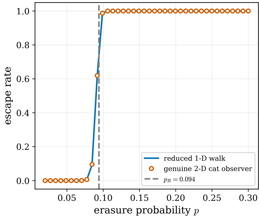
(a) UZQ faithfulness: 2-D cat map = 1-D reduction
