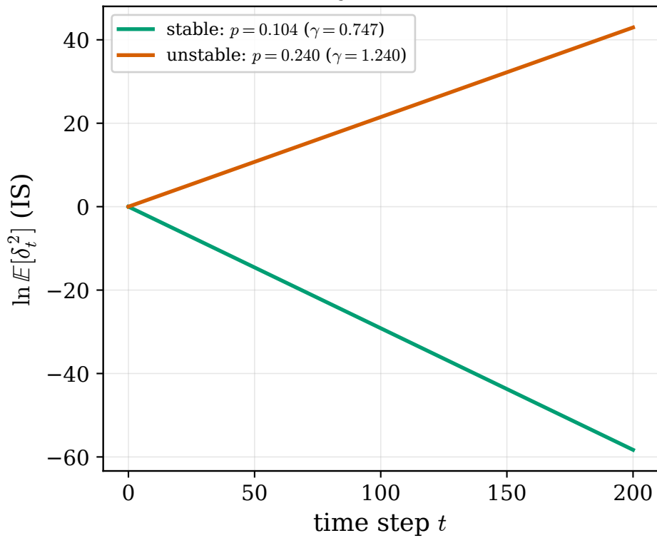
(b) UZQ sufficiency at R = h_R + 0.5 , p_c = 0.174
