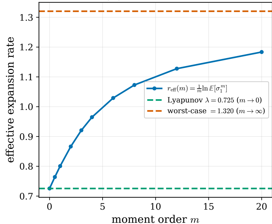
(a) Henon: r_{\text{eff}}(m) rises Lyapunov \rightarrow restoration
