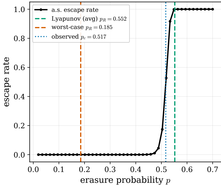
(b) a.s. escape follows the Lyapunov average
