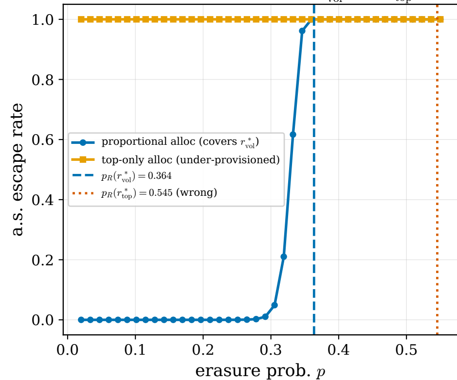
(a) RATE condition uses r_{\text{vol}}^* , not r_{\text{top}}^*
