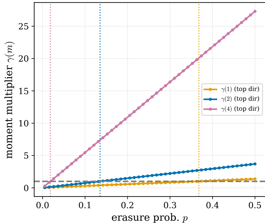
(b) MOMENT threshold p_c(m) = e^{-m r_{\text{top}}^*}
