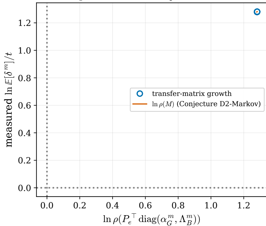
(b) spectral-radius conjecture is exact
