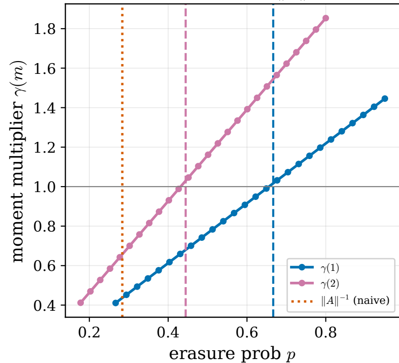
shear c=3: \rho = 1.50 , \|A\| = 3.53
