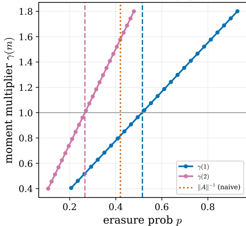
rot+stretch: \rho = 1.94 , \|A\| = 2.38
