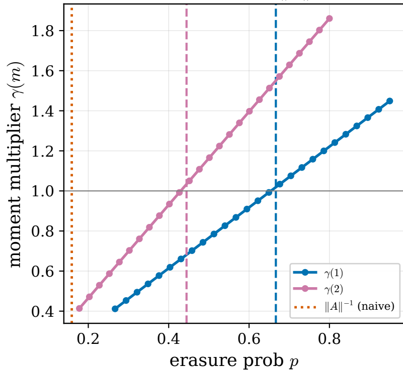
shear c=6: \rho = 1.50 , \|A\| = 6.29
