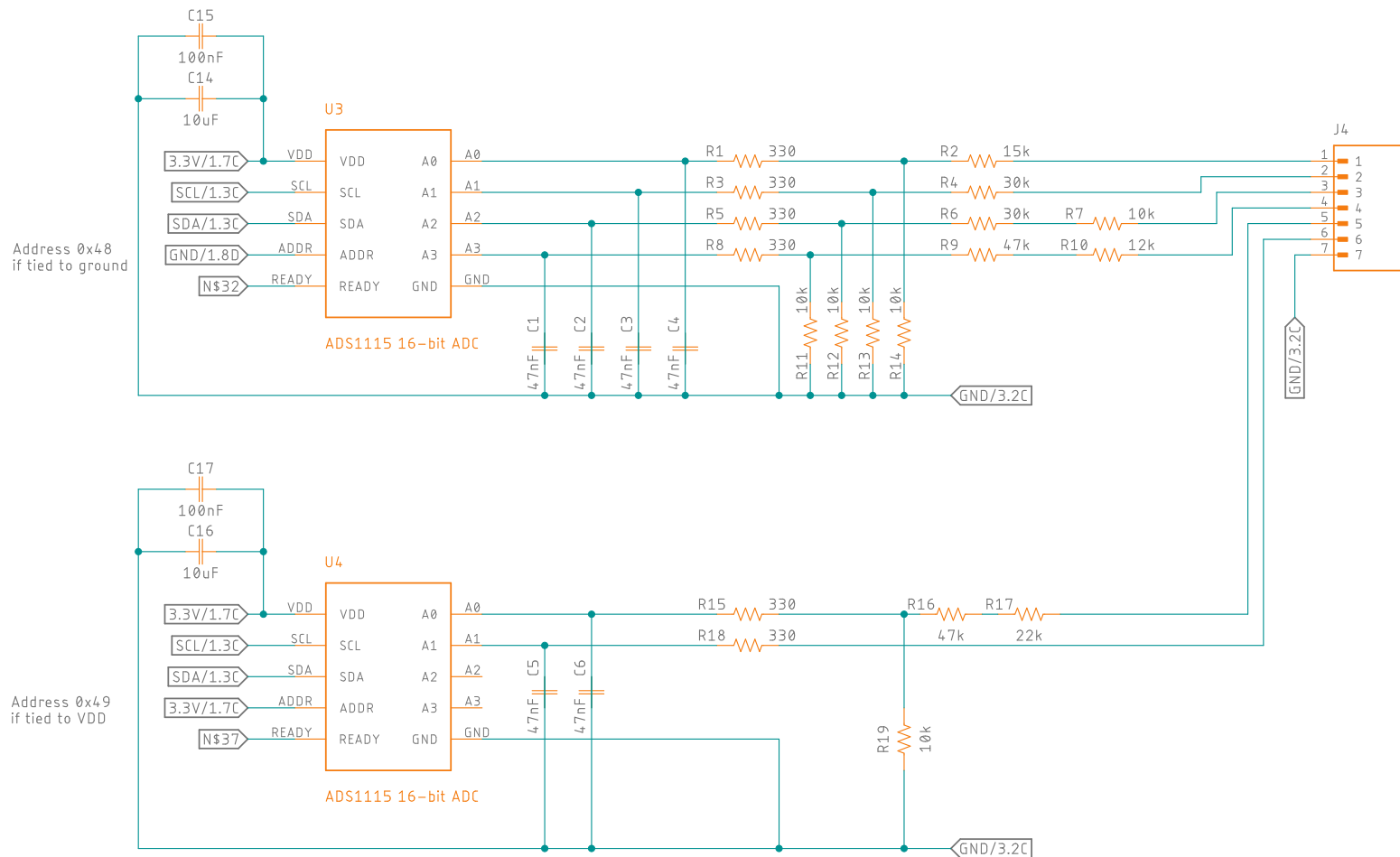
6S LiPo voltage measurement with ADS1115 Resistor divider network:
