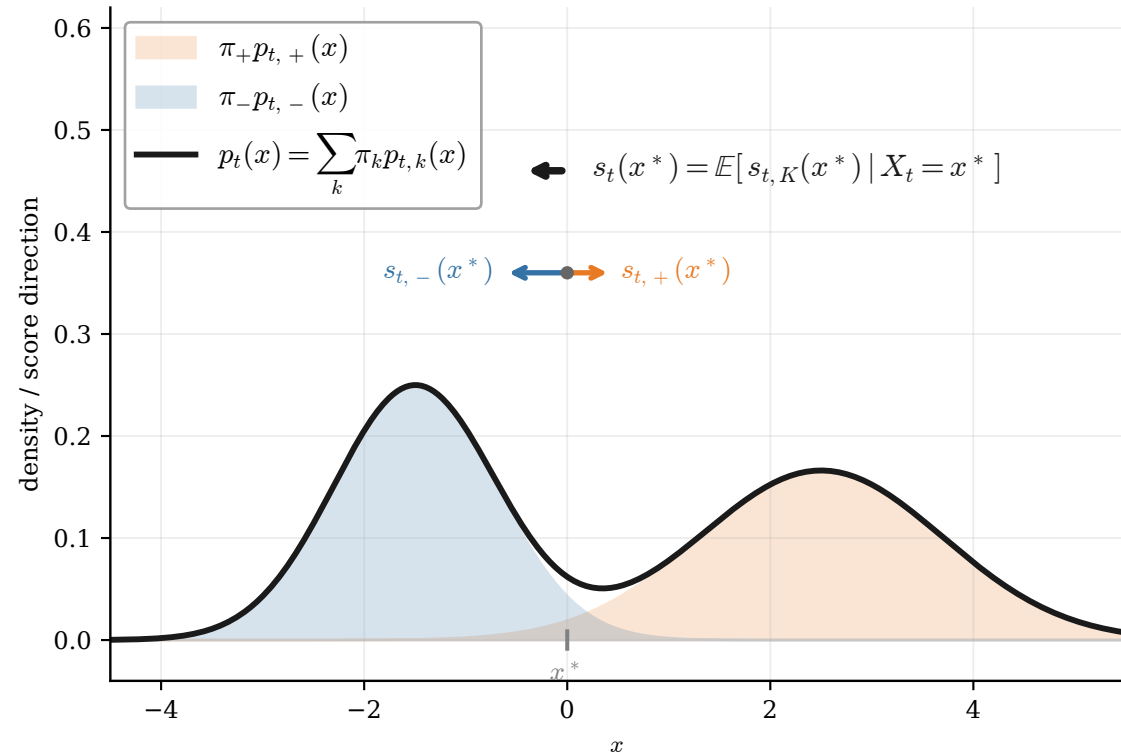
(a) Diffusion: score is a posterior average
