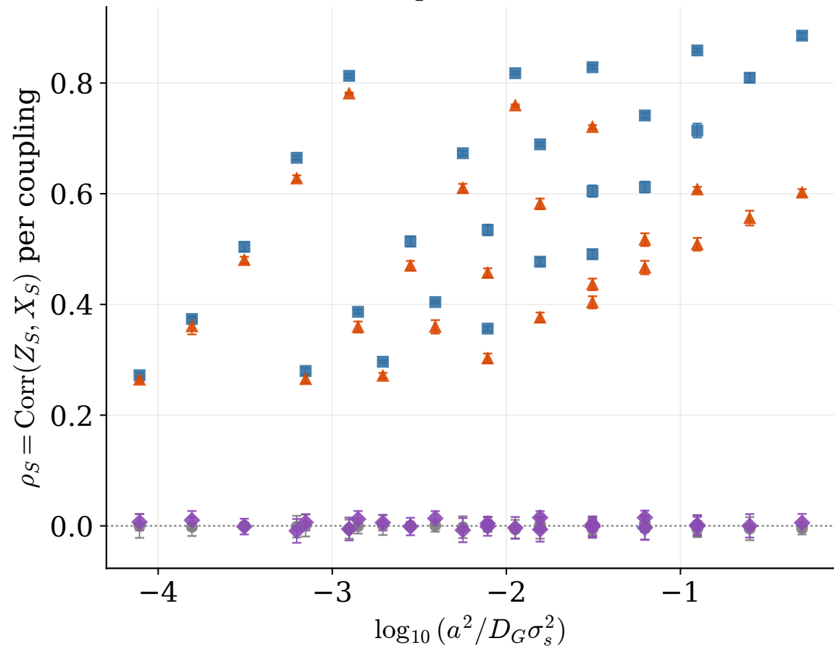
(a) Semantic endpoint correlation vs \ell SNR
