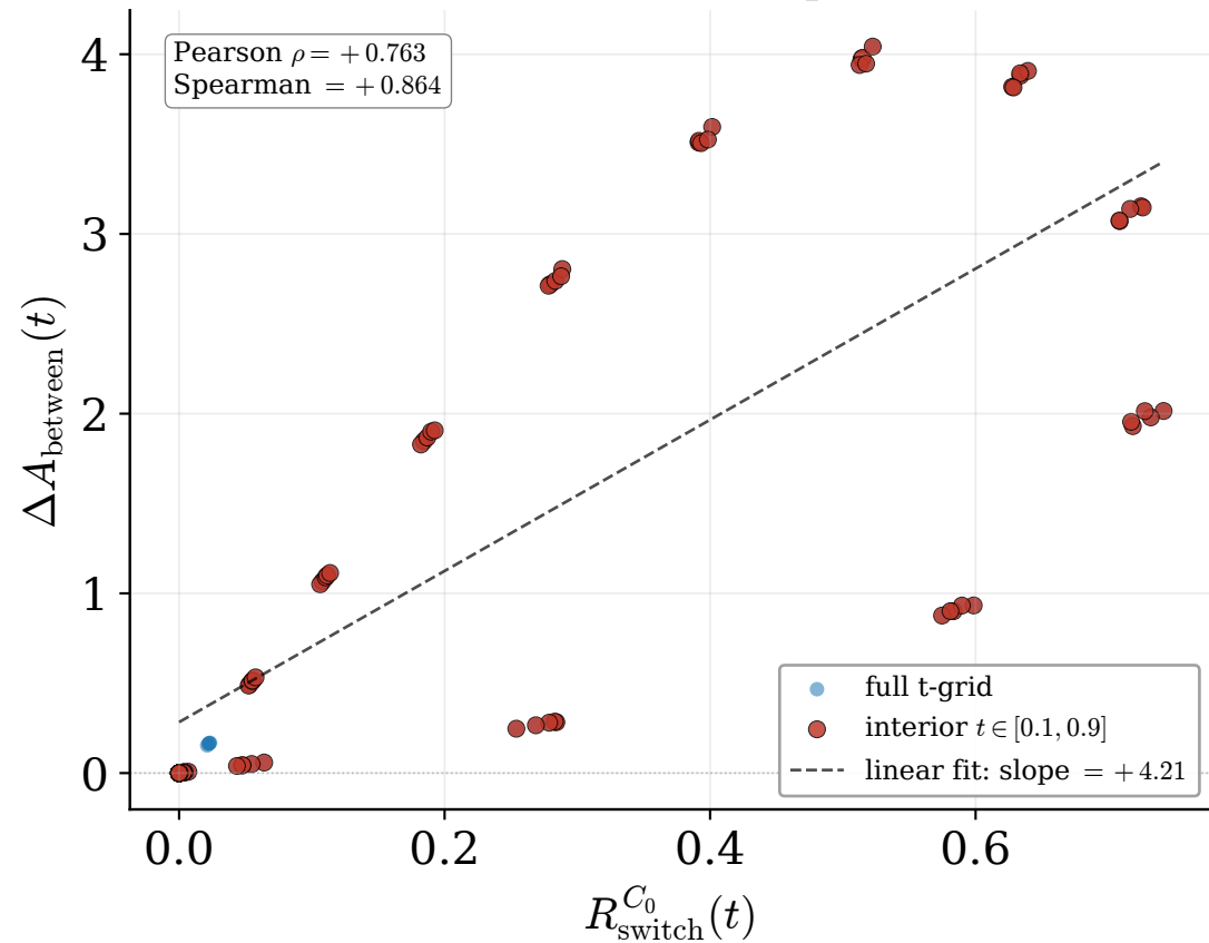
(a) coarse K (XOR superclass)
