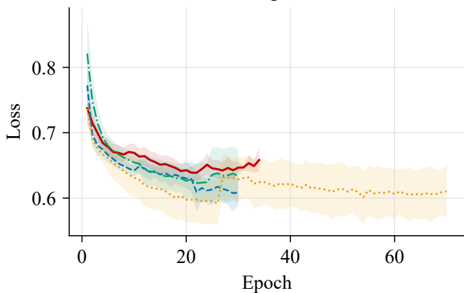
Training Loss
