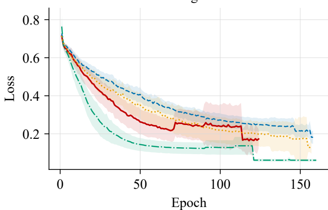
Training Loss
