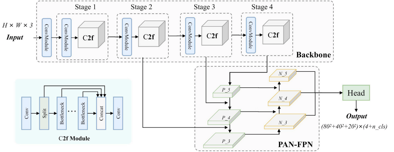
Fig. 5 – The architecture of the YOLOv8.
