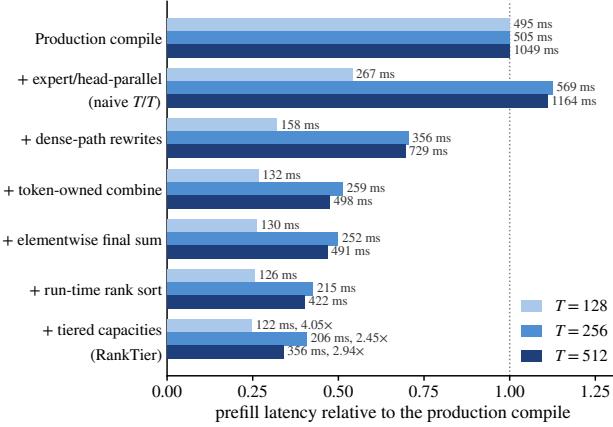
Figure 3. Prefill latency of the seven programs relative to the production compilation at the same chunk length, with the latency of each program and the speedup of RankTier.
