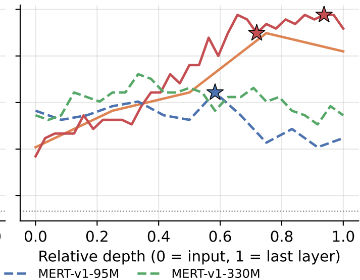
Task 2: market
