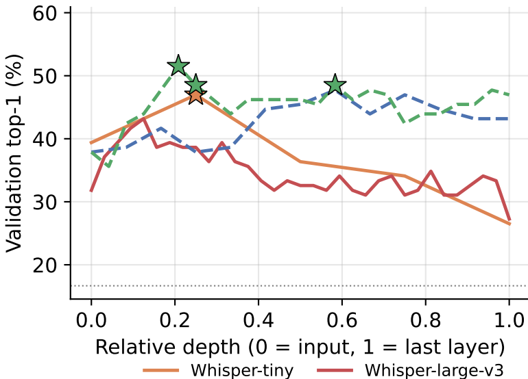
Task 1: decade
