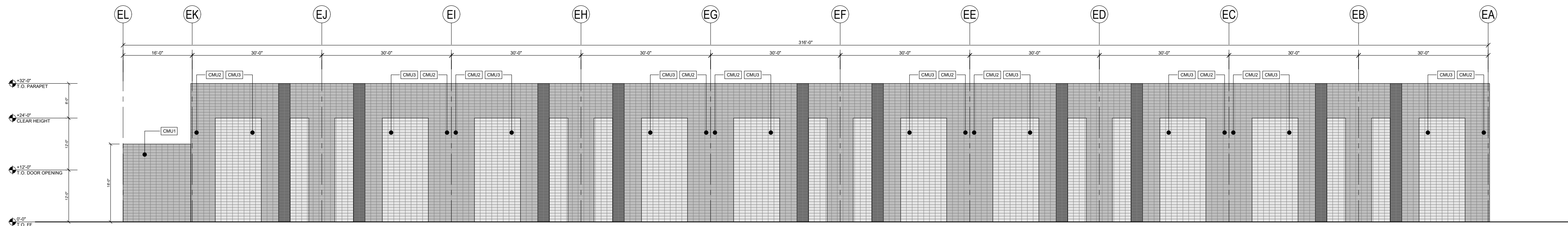
01 NORTH ELEVATION - BUILDING E SCALE: 1/16" = 1'-0"
