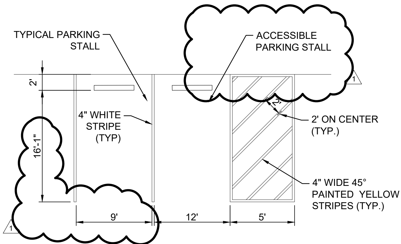
2 ACCESSIBLE PARKING LAYOUT DETAIL Scale: NTS
