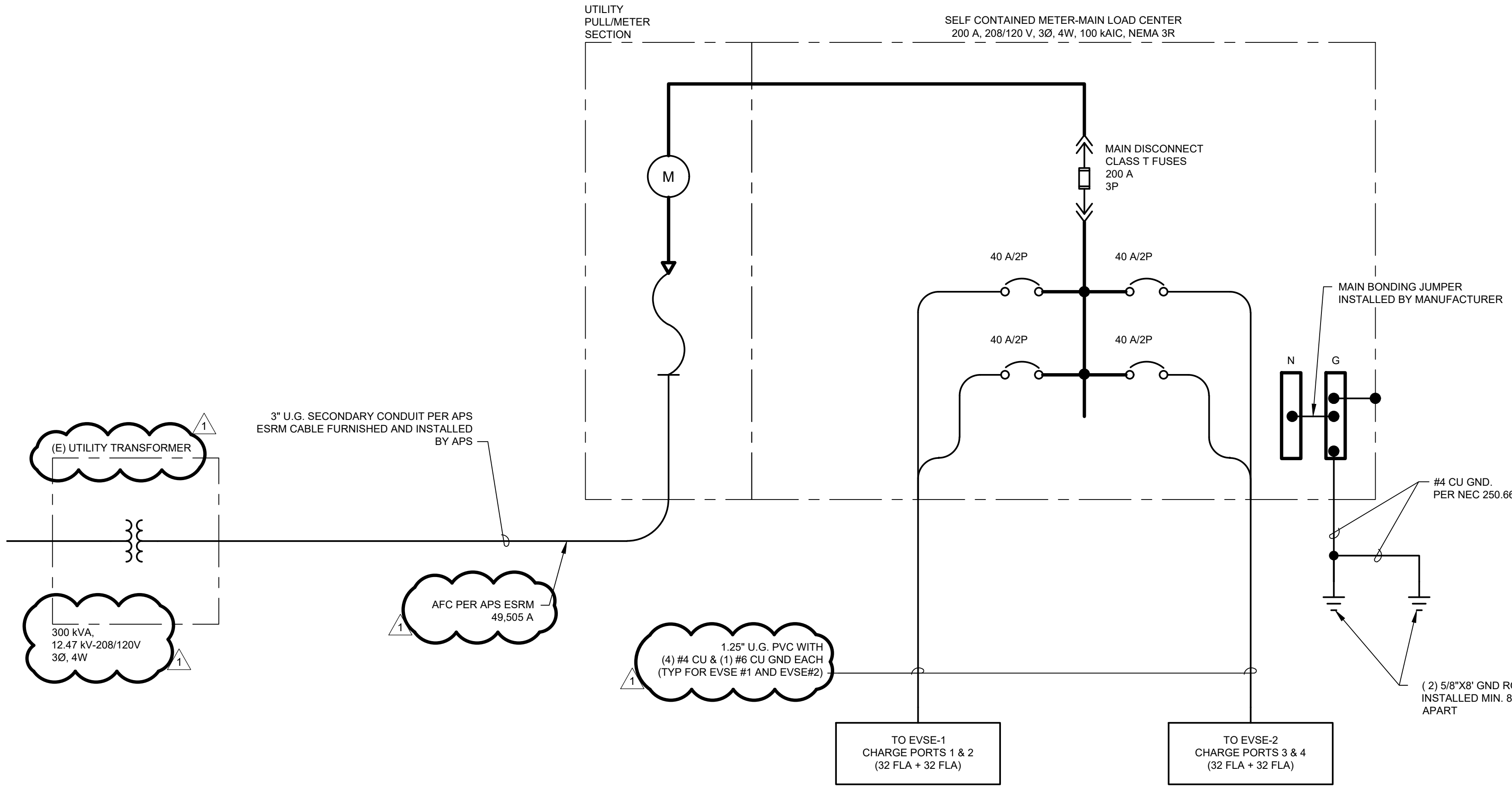
ONE-LINE DIAGRAM
