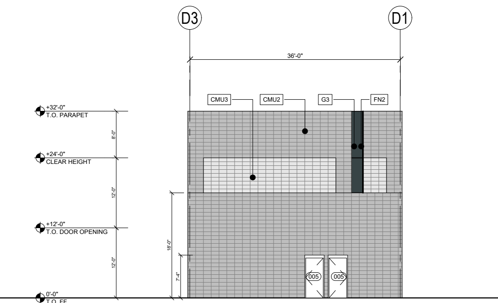
04 SOUTH ELEVATION - BUILDING D SCALE: 1/16" = 1'-0"
