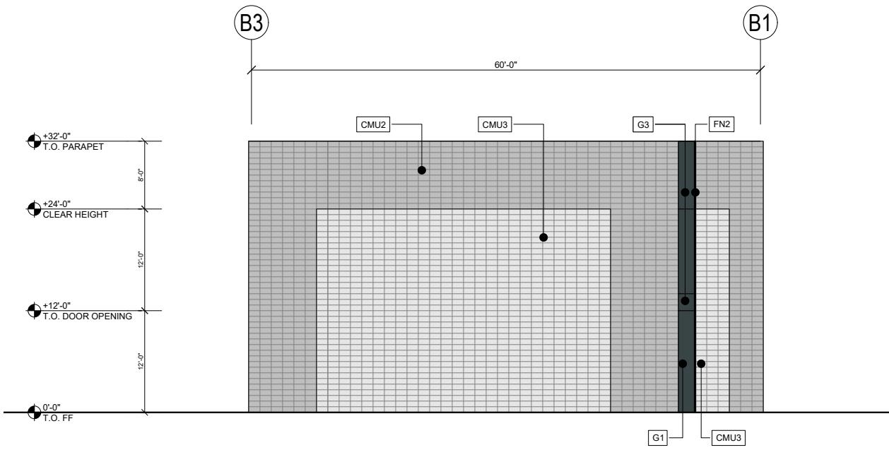
04 SOUTH ELEVATION - BUILDING B SCALE: 1/16" = 1'-0"
