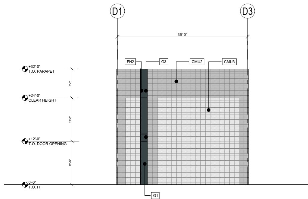
03 NORTH ELEVATION - BUILDING D SCALE: 1/16" = 1'-0"
