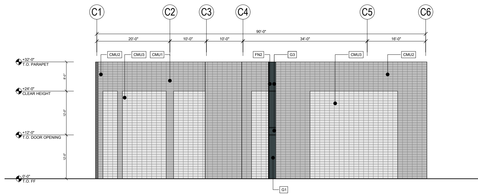
01 SOUTH ELEVATION - BUILDING C SCALE: 1/16" = 1'-0"
