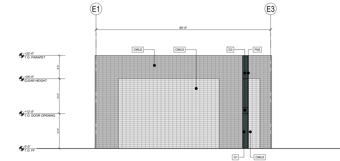
03 WEST ELEVATION - BUILDING E SCALE: 1/16" = 1'-0"
