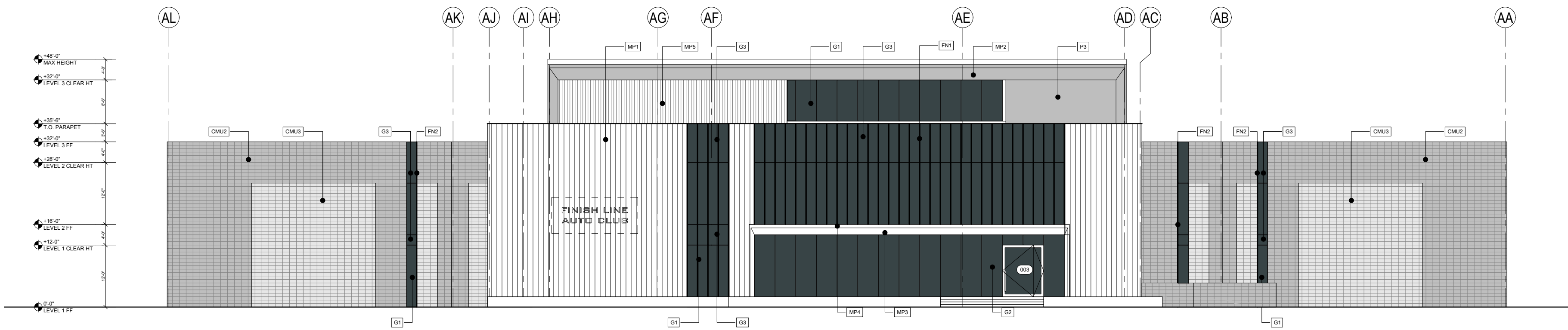
04 EAST ELEVATION - BUILDING A SCALE: 1/16" = 1'-0"
