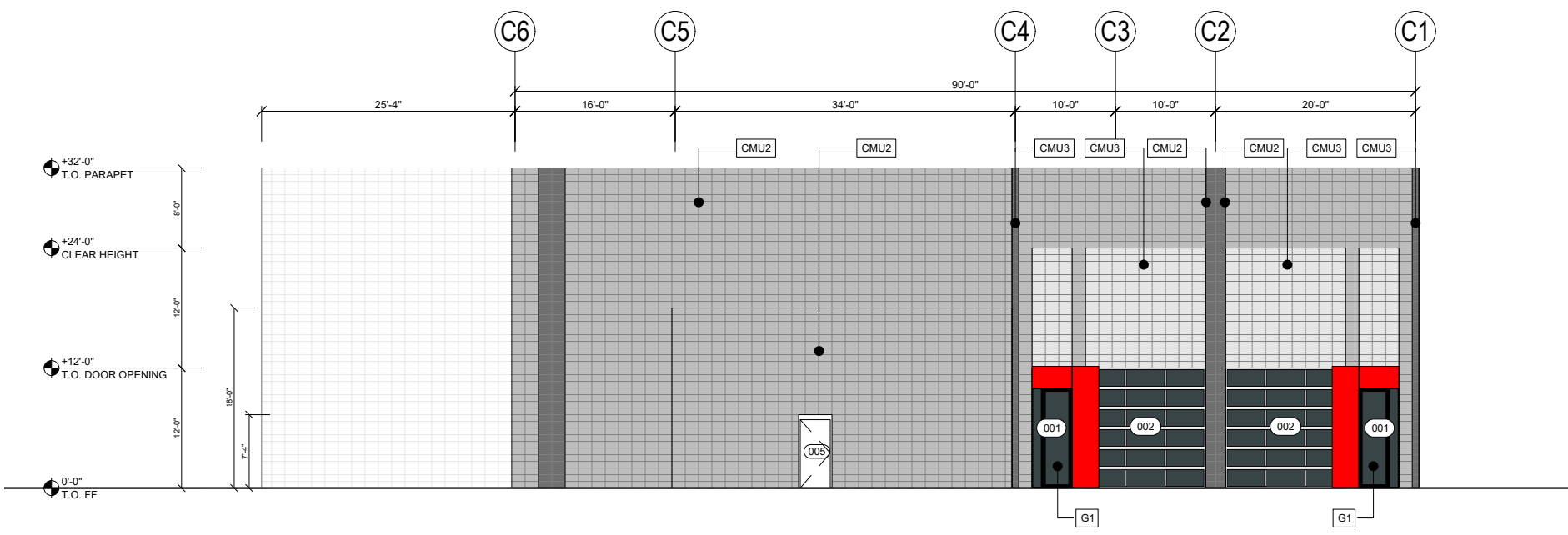
03 NORTH ELEVATION - BUILDING C SCALE: 1/16" = 1'-0"
