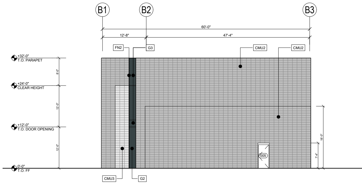
03 NORTH ELEVATION - BUILDING B SCALE: 1/16" = 1'-0"
