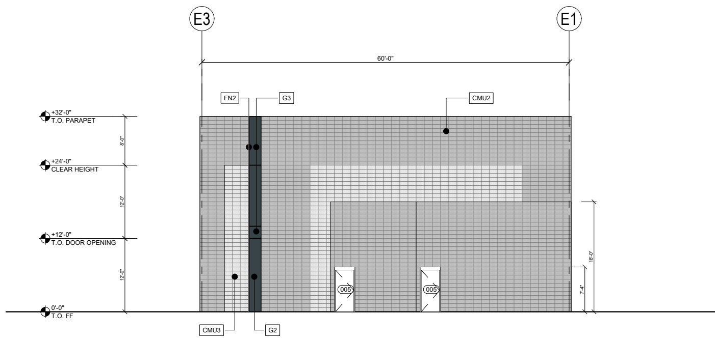
04 EAST ELEVATION - BUILDING E SCALE: 1/16" = 1'-0"
