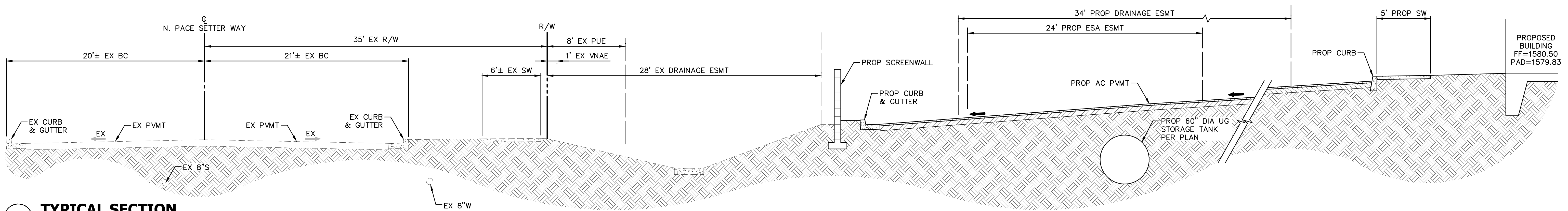
A TYPICAL SECTION
