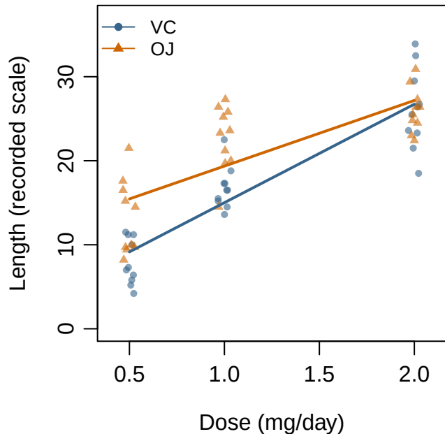
Interaction: two slopes
