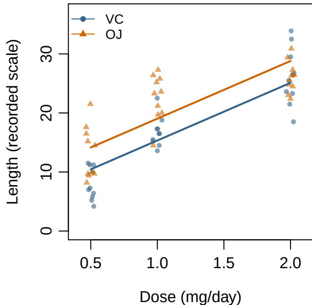
Additive: common slope
