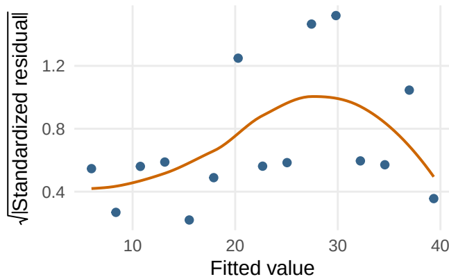
Scale-location
