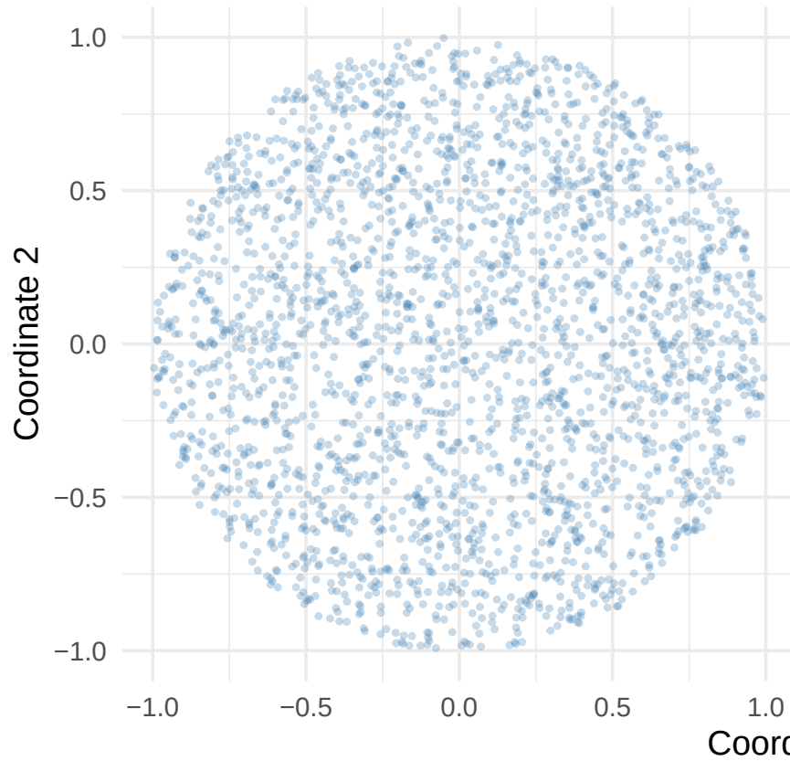
Interior: unit disk
