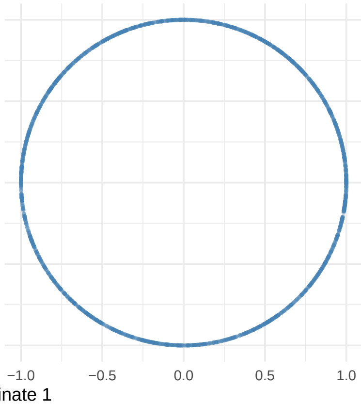
Surface: unit circle
