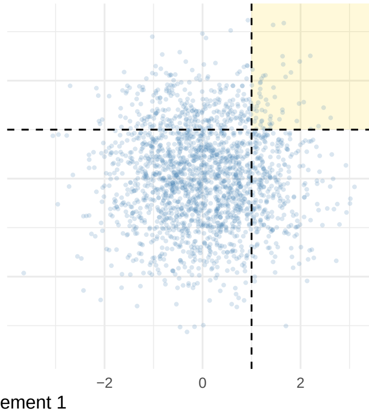
Independent
