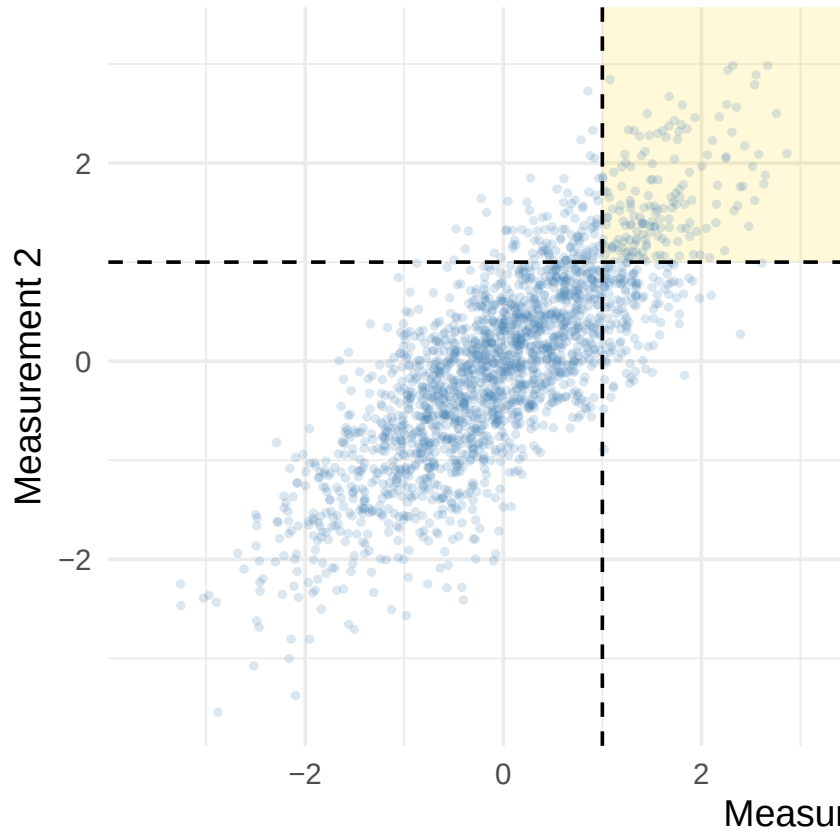
Correlation 0.8
