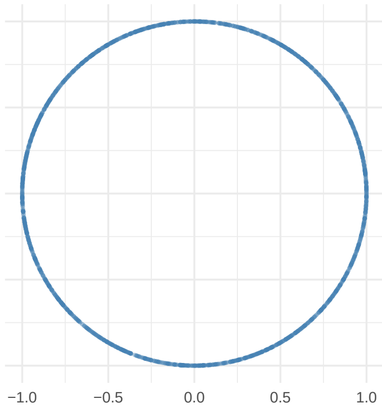
Surface: unit circle
