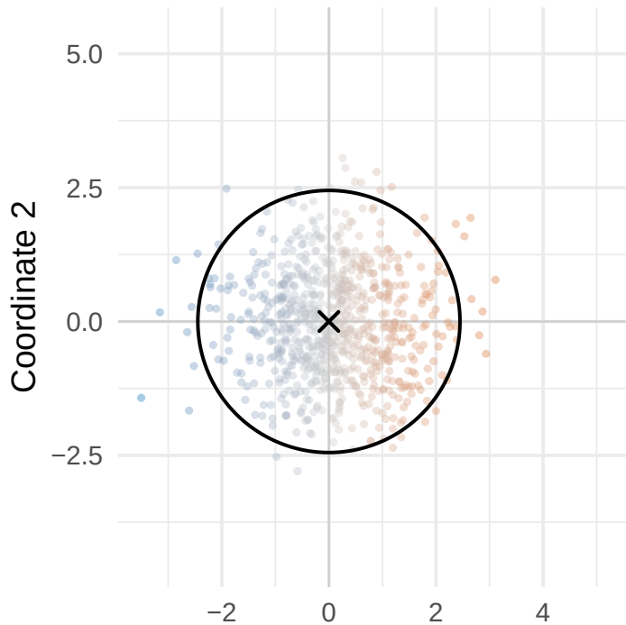
1. Independent normals
